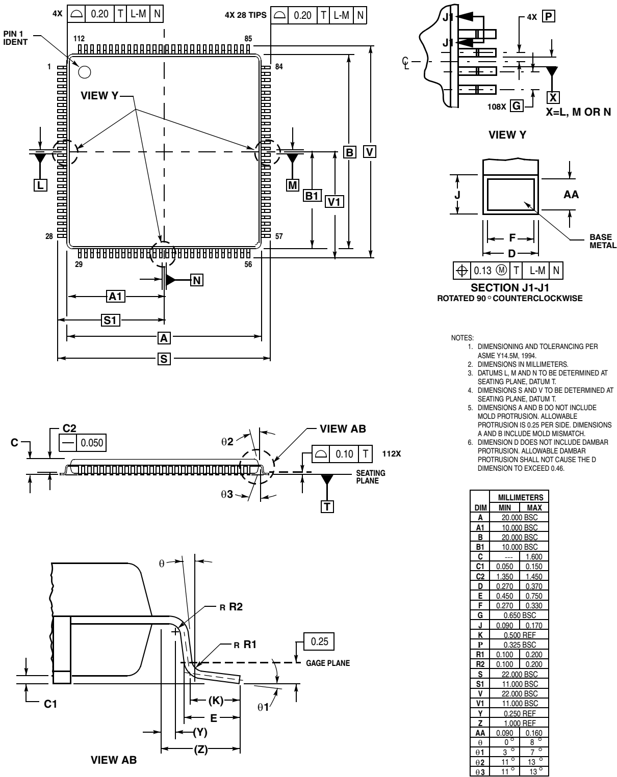
Figure 3-3. 112-pin QFP Mechanical Dimensions (case no. 987)
