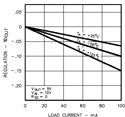
FIGURE 1. LOAD REGULATION
