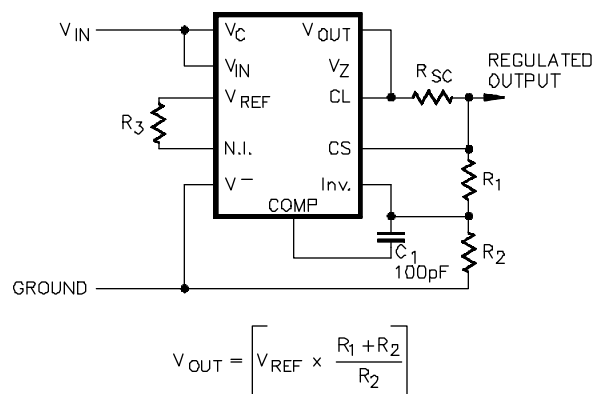
FIGURE 8 - BASIC HIGH VOLTAGE REGULATOR V_{OUT} = 7V \text{ TO } 37V
