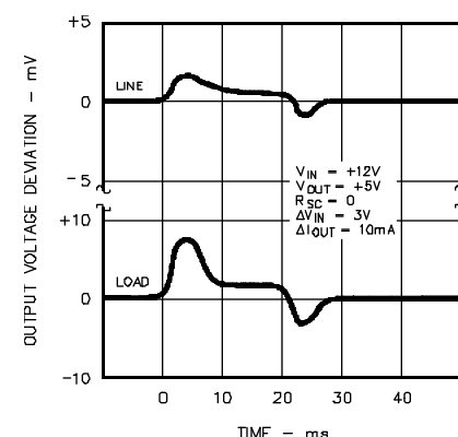
FIGURE 6. TRANSIENT RESPONSE
