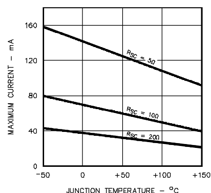
FIGURE 3. CURRENT LIMITING CHARACTERISTICS
