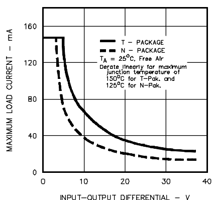
FIGURE 2. MAXIMUM LOAD CURRENT
