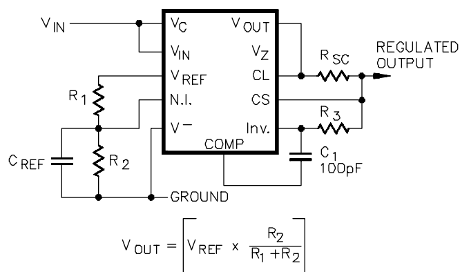
FIGURE 7 - BASIC LOW VOLTAGE REGULATOR V_{OUT} = 2V \text{ TO } 7V
