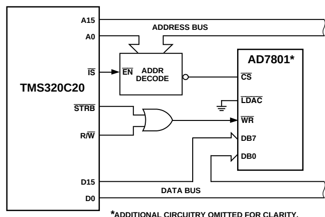
Figure 30. AD7801-TMS320C20 Interface
