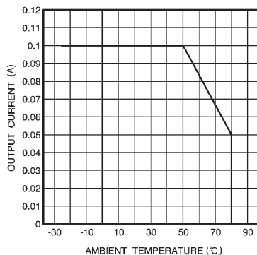
Fig.14 Derating curve
