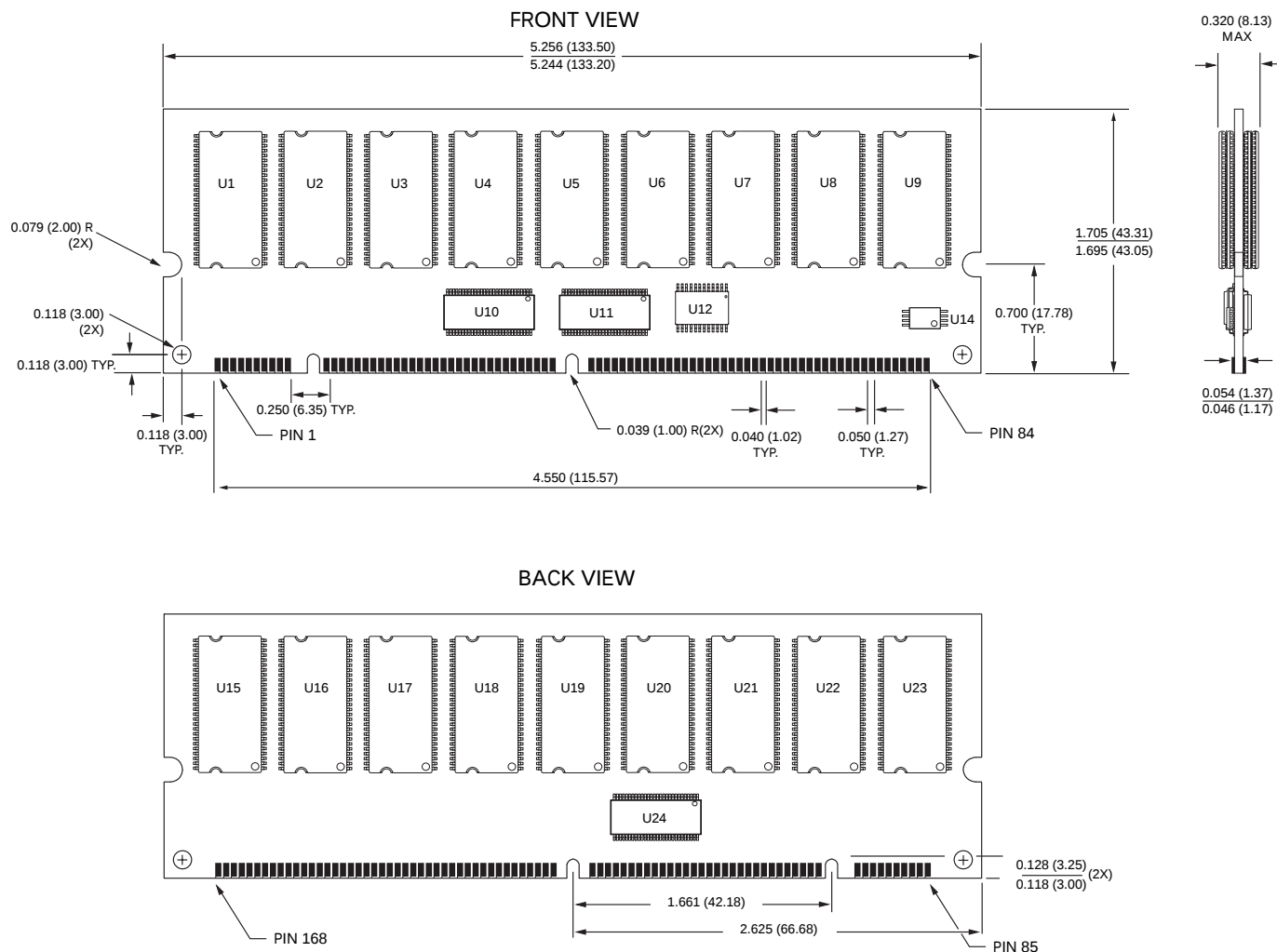
Figure 12: 168-Pin DIMM Dimensions – Standard PCB
