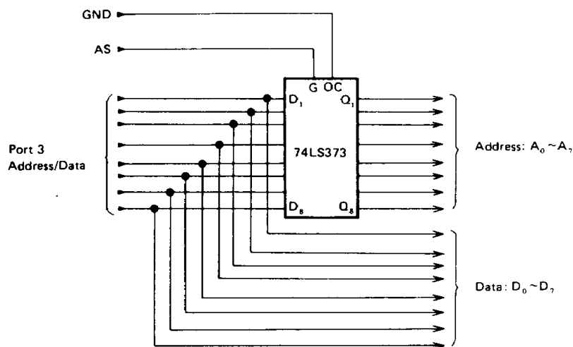
Figure 19 Latch Connection
