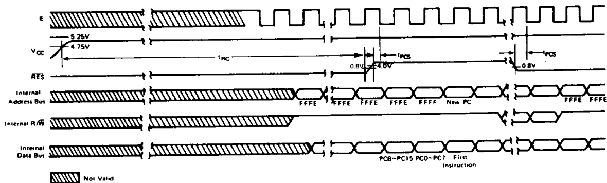
Figure 11 Reset Timing
