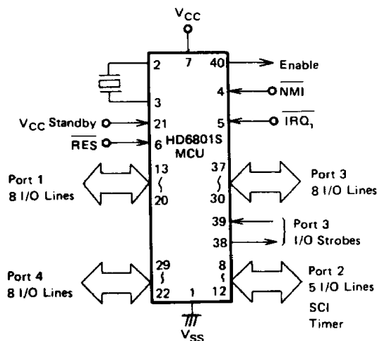
Figure 16 HD6801S MCU Single-Chip Mode
