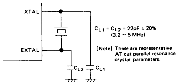
Figure 12 Crystal Interface
