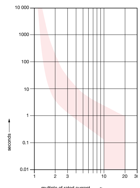
Tripping Characteristic D
