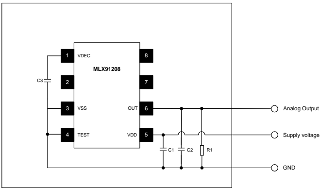
Figure 8: Diagnostic low/ Pull-down resistors
