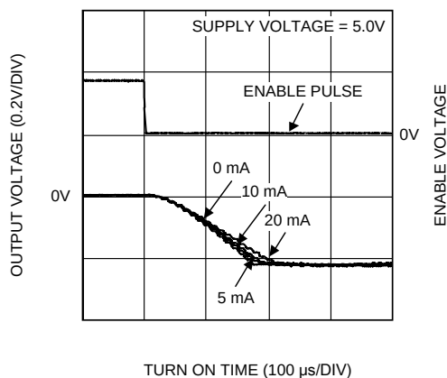
Figure 12. Turnon Time
