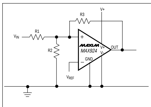
Figure 4. External Hysteresis
