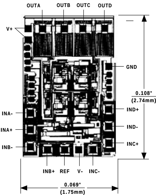
MAX924
