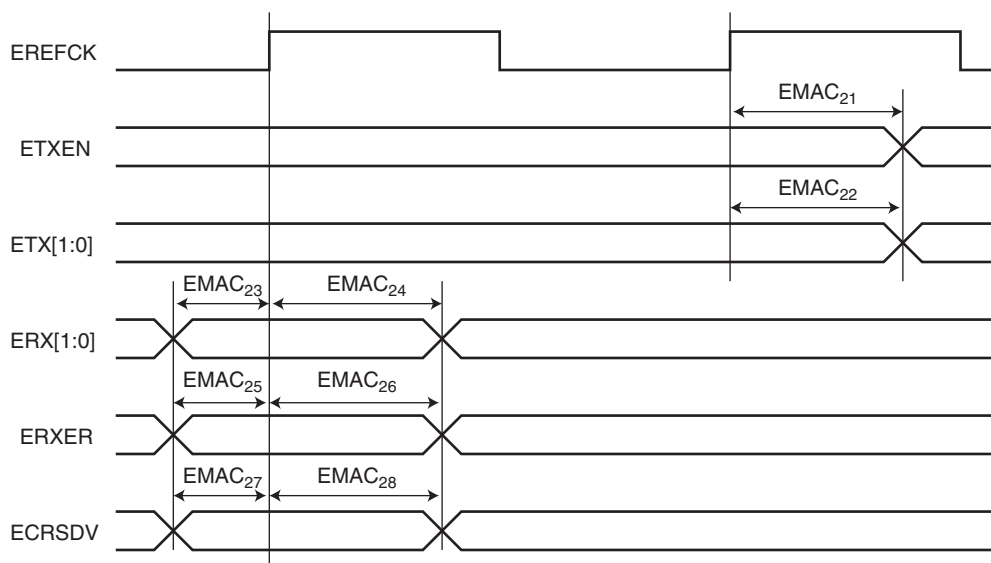
Figure 43-5. EMAC RMII Mode
