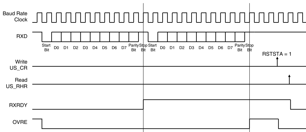
Figure 34-21. Receiver Status
