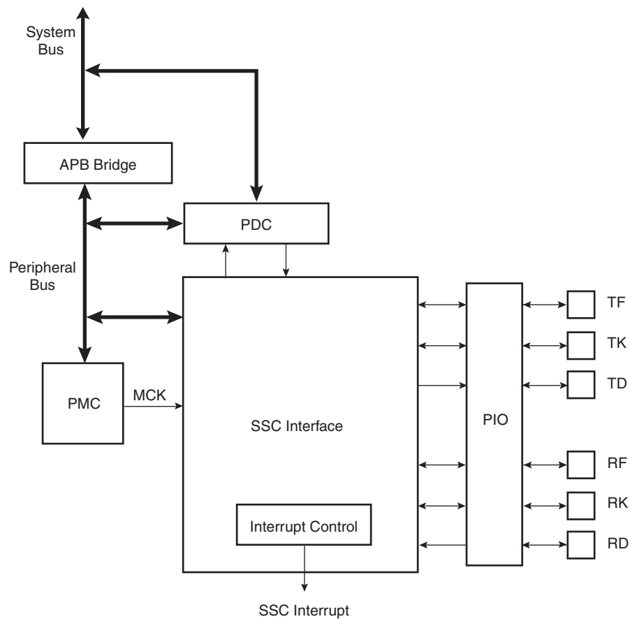
Figure 35-1. Block Diagram
