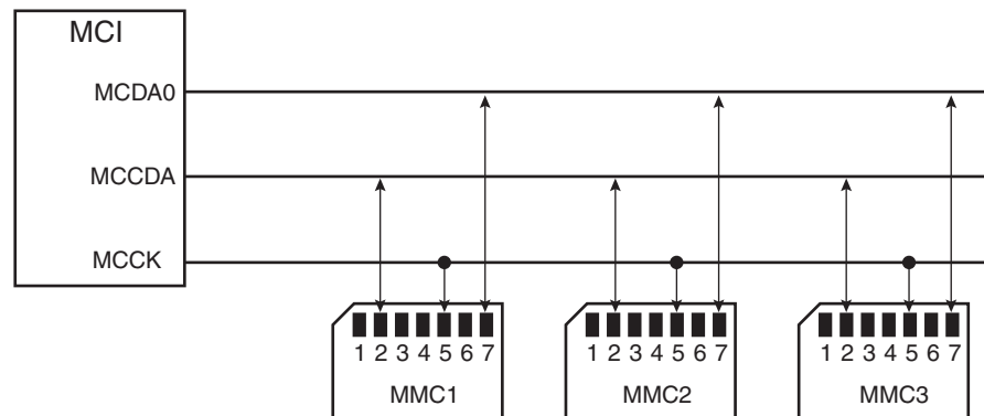
Figure 37-4. MMC Bus Connections (One Slot)
