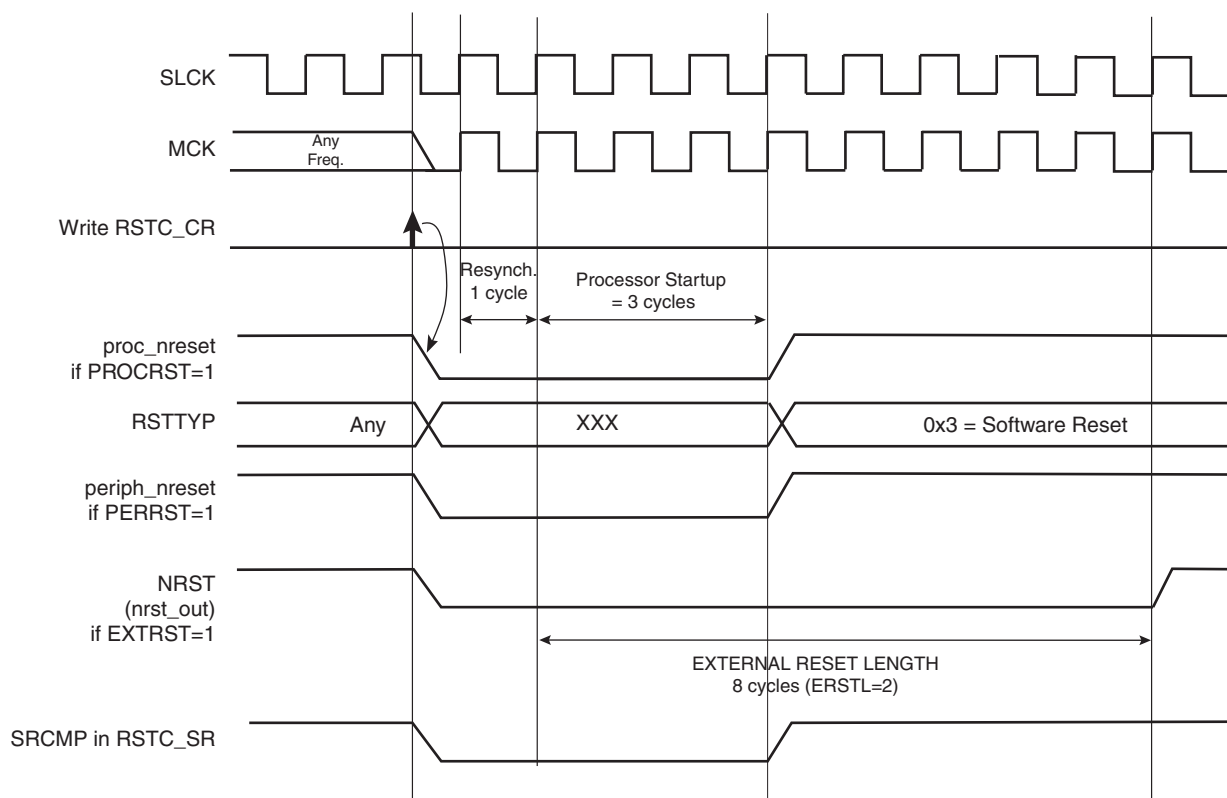
Figure 15-8. Software Reset
