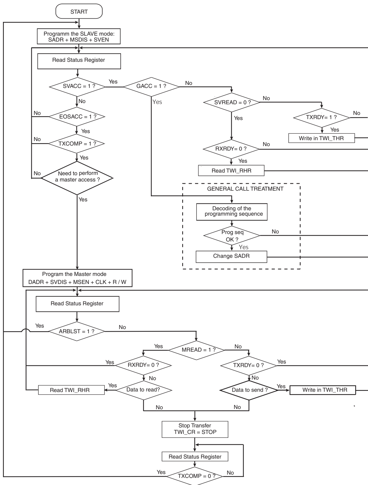
Figure 33-23. Multi-master Flowchart
