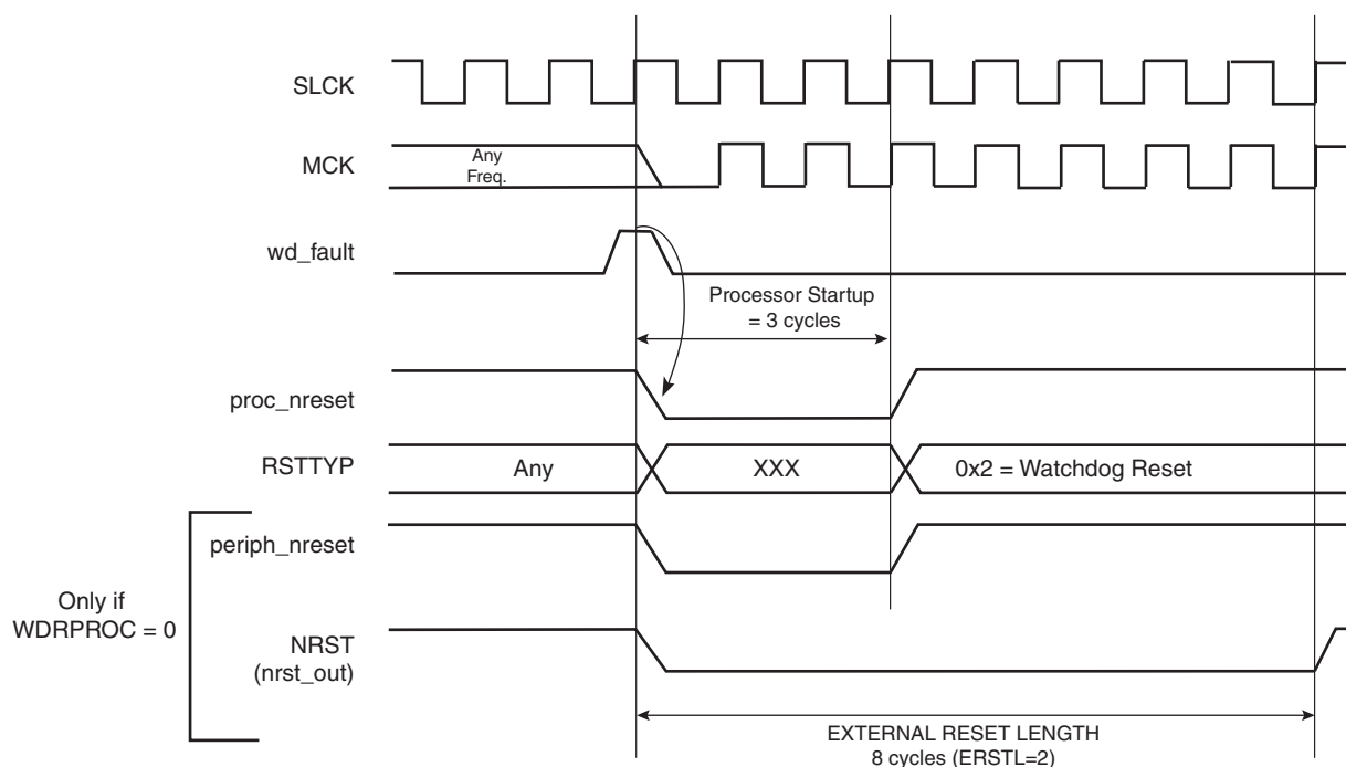
Figure 15-9. Watchdog Reset
