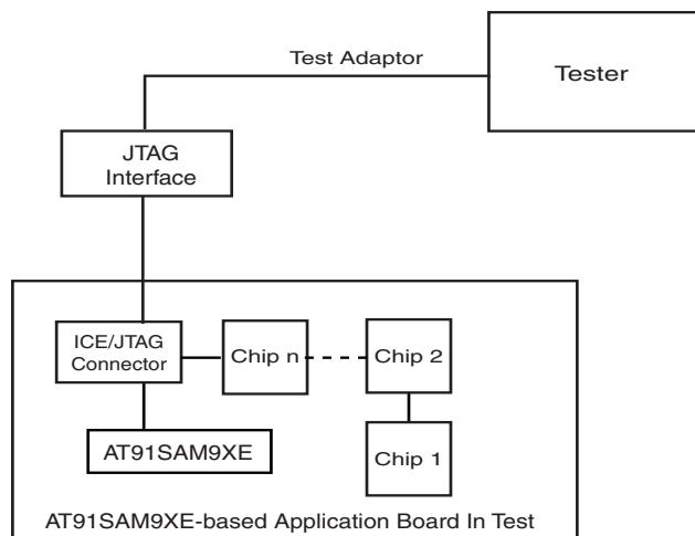
Figure 12-3. Application Test Environment Example
