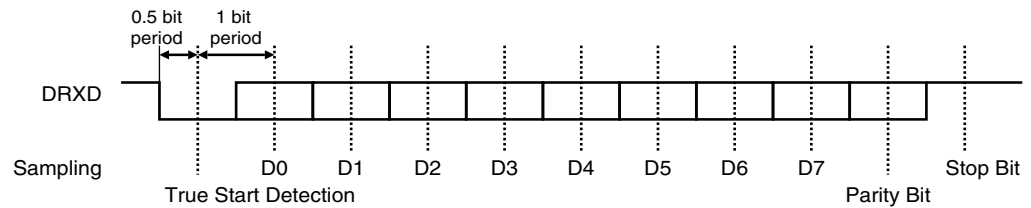
Figure 30-5. Character Reception
