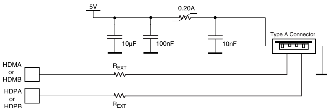
Figure 40-4. Board Schematic to Interface UHP Device Controller
