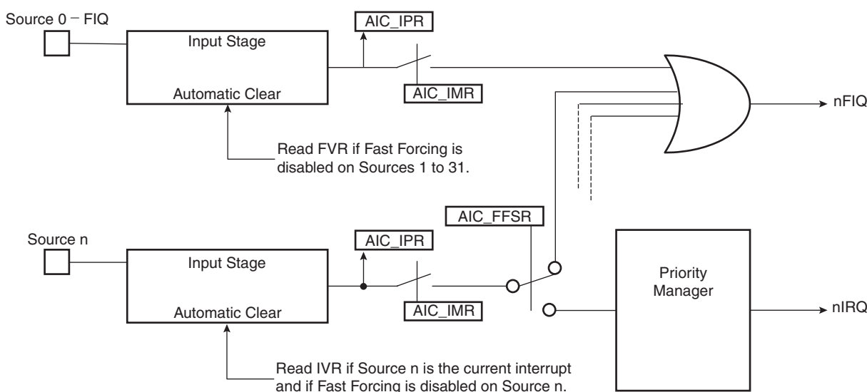
Figure 29-10. Fast Forcing
