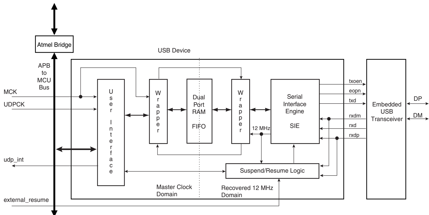
Figure 39-1. Block Diagram
