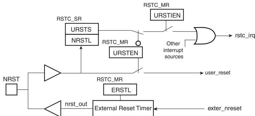
Figure 15-2. NRST Manager
