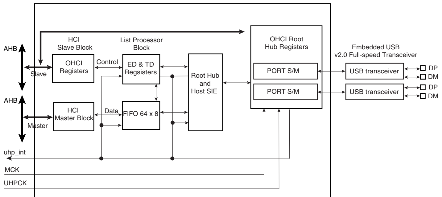
Figure 40-1. Block Diagram
