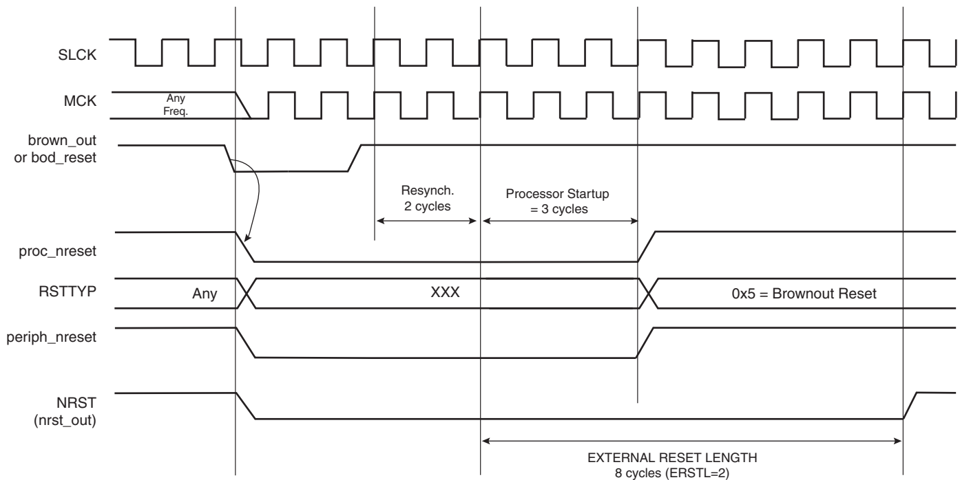
Figure 15-7. Brownout Reset State
