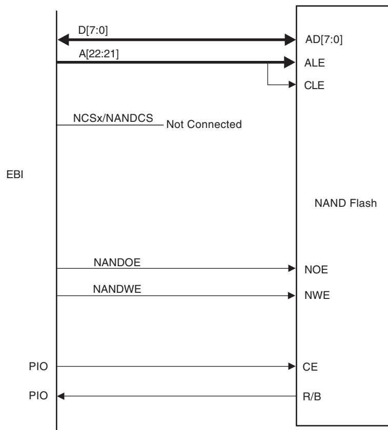
Figure 22-7. NAND Flash Application Example
