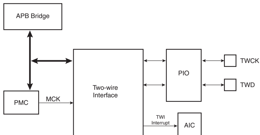
Figure 33-1. Block Diagram
