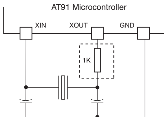
Figure 27-4. Typical Crystal Connection
