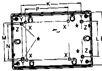
PLAN VIEW OF BASE AND TOP
