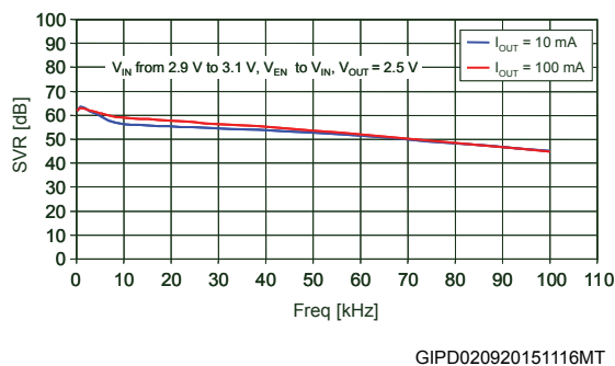
Figure 20. Supply voltage rejection vs. frequency ( V_{OUT} = 2.5 V)
