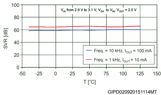
Figure 18. Supply voltage rejection vs. temperature ( V_{OUT} = 2.5 V)
