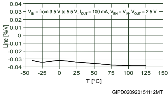
Figure 16. Line regulation V_{OUT} = 2.5 V
