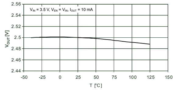
Figure 5. V_{OUT} accuracy
