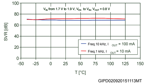
Figure 17. Supply voltage rejection vs. temperature ( V_{OUT} = 0.8 V)
