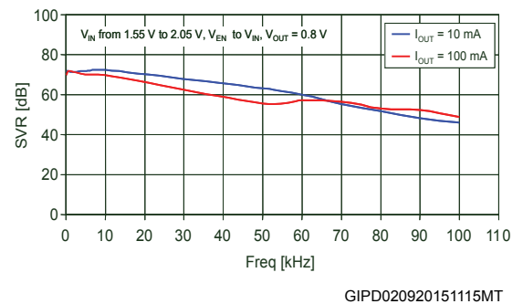
Figure 19. Supply voltage rejection vs. frequency ( V_{OUT} = 0.8 V)
