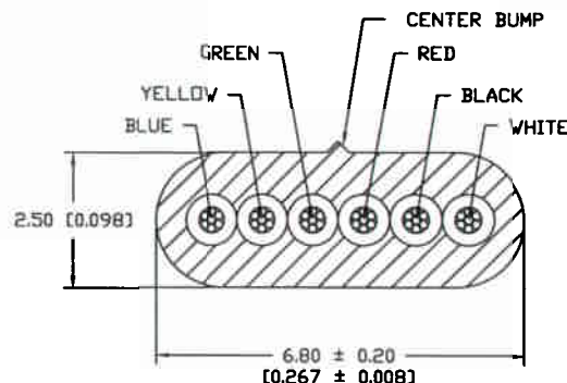
6 CONDUCTOR CABLE
