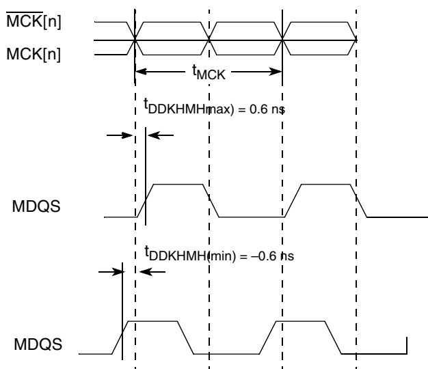
Figure 4. Timing Diagram for t_{\text{DDKMH}}
