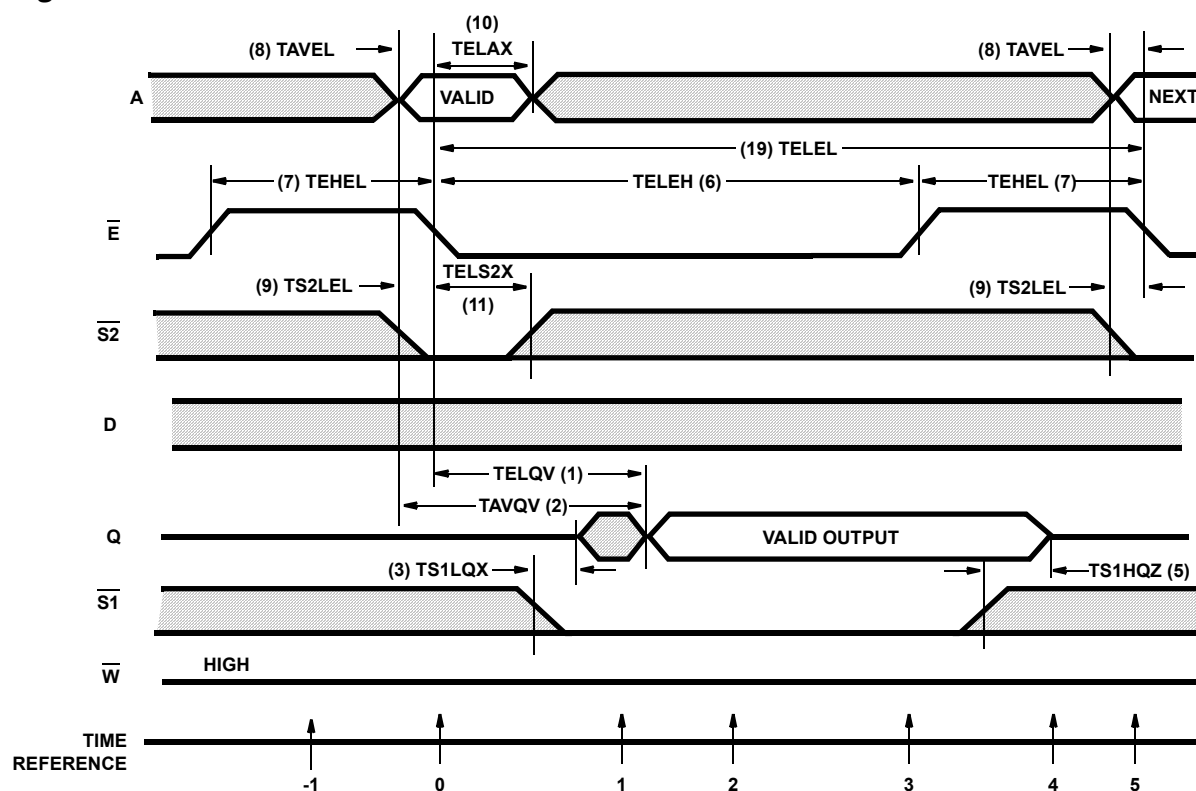
FIGURE 1. READ CYCLE
