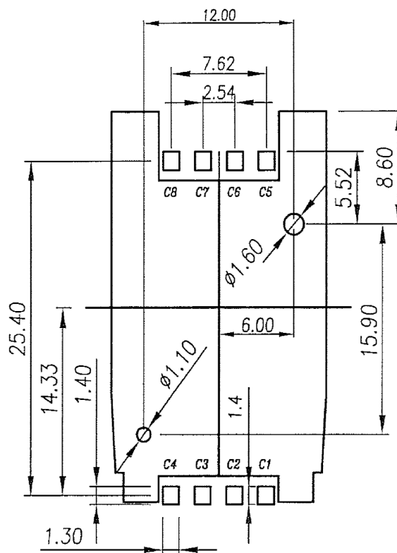
PCB LAYOUT RECOMMENDED
