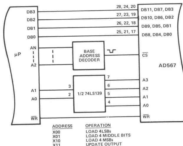
Figure 6. Addressing for 4-Bit Microprocessor Interface
