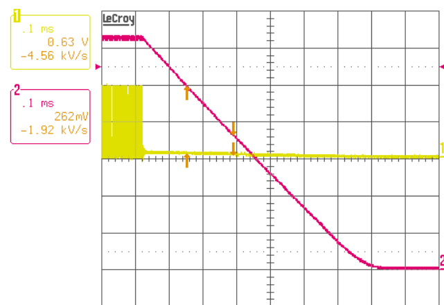
FIGURE 55. 1-PHASE GPU MODE SHUT DOWN, V_{IN} = 8V , I_O = 1A , V_{ID} = 1.2375V , Ch1: PHASE1, Ch2: V_O
