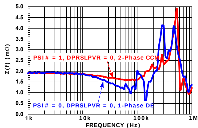
FIGURE 53. REFERENCE DESIGN FIM RESULT
