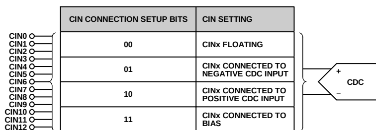
Figure 28. Input Mux Configuration Options
