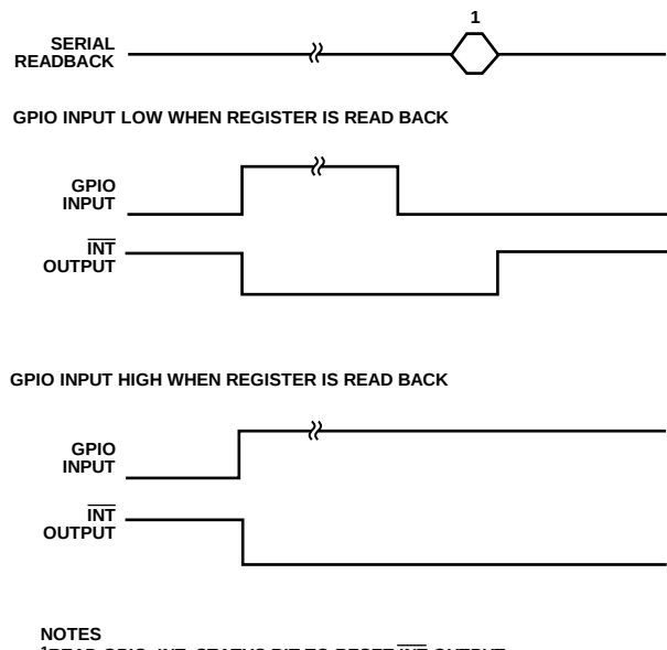
Figure 45. Example of INT Output Controlled by the GPIO Input (GPIO_SETUP = 01, GPIO_INPUT_CONFIG = 11)
