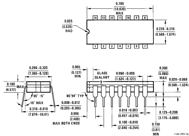
Ceramic Dual-In-Line Package (J) Order Number LM110J/883 NS Package Number J14A
