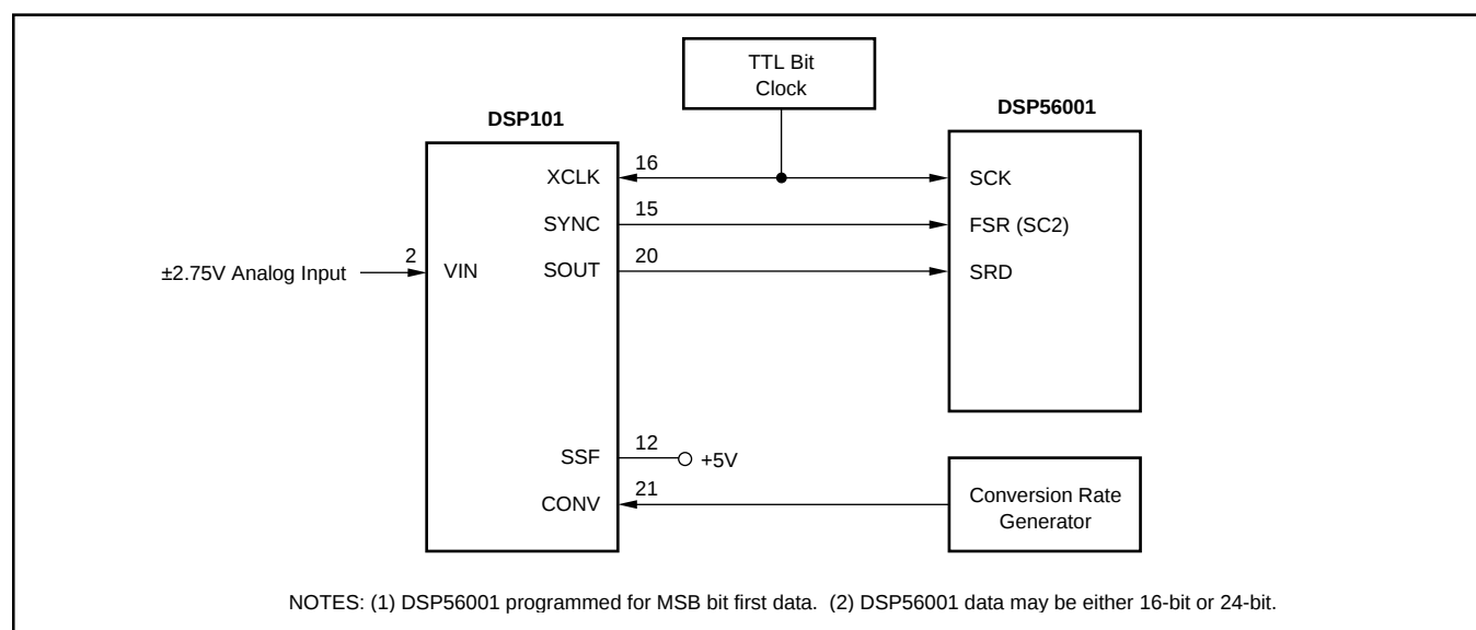
FIGURE 18. Using DSP101 with DSP56001.
