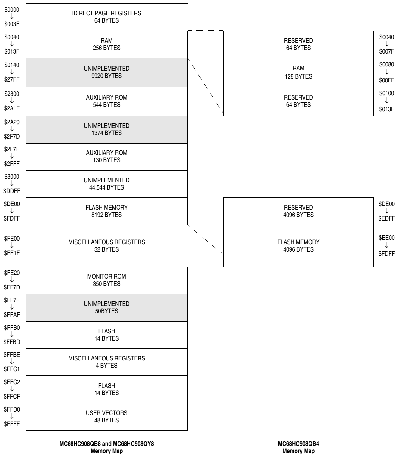
Figure 2-1. Memory Map
