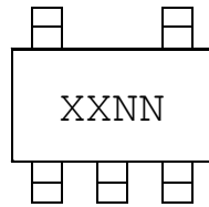
5-Lead SOT-23 (MCP6561, MCP6561R)
