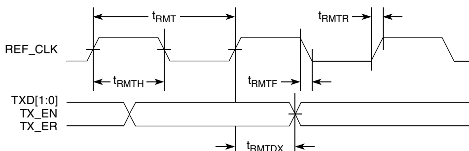
Figure 20. RMI Transmit AC Timing Diagram
