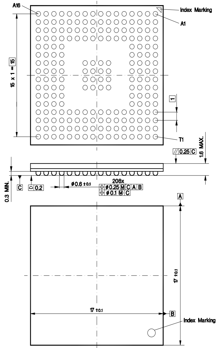
Figure 5-1 P-LBGA-208-2 Package
