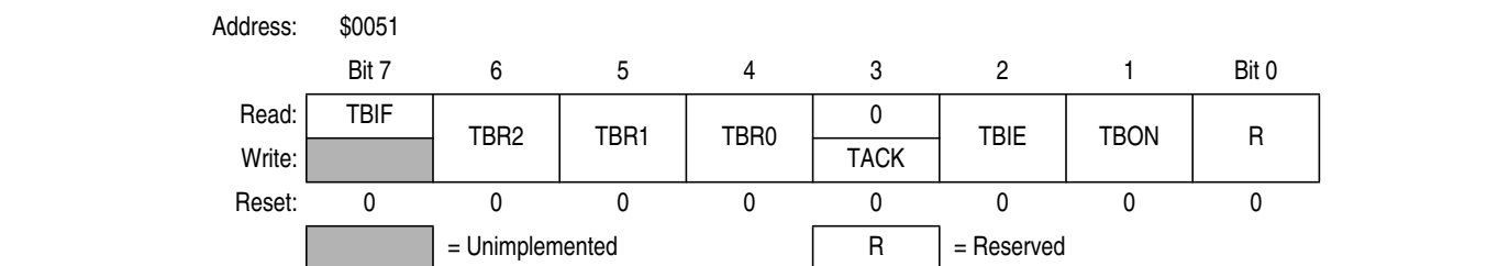
Figure 10-2. Timebase Control Register (TBCR)
