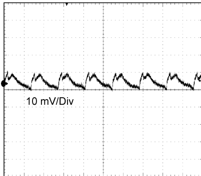
Figure 37. Output Ripple
