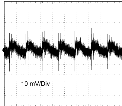
Figure 38. Output Ripple
