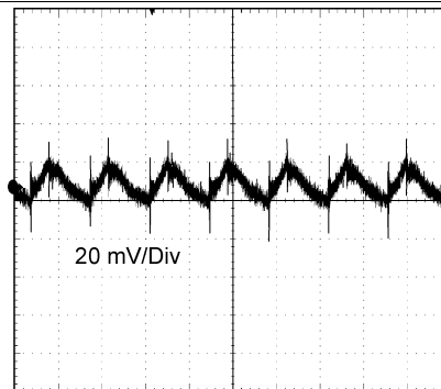
Figure 34. Output Ripple
