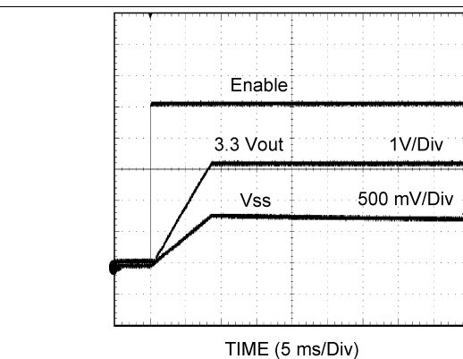
Figure 44. 3.3 V OUT Soft-Start
