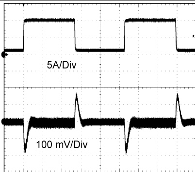
Figure 37. Output Ripple
