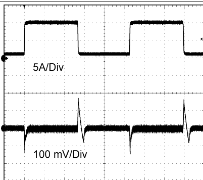
Figure 39. Transient Response
