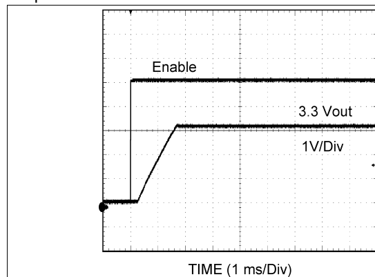
Figure 43. 3.3 V OUT Soft-Start
