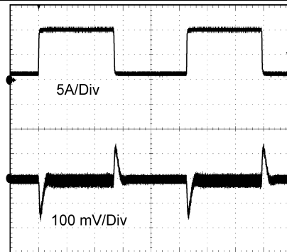
Figure 38. Output Ripple
