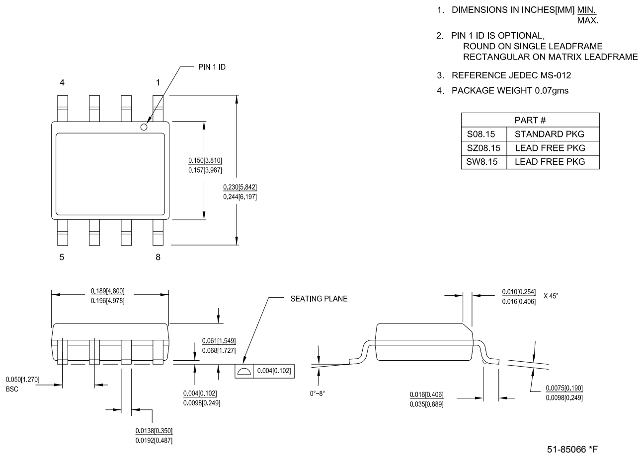
Figure 12. 8-pin (150-mil) SOIC Package Outline
