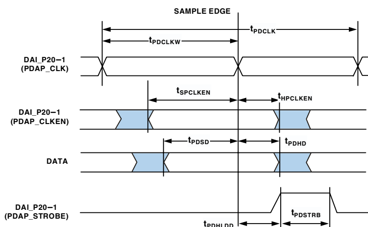
Figure 19. PDAP Timing
