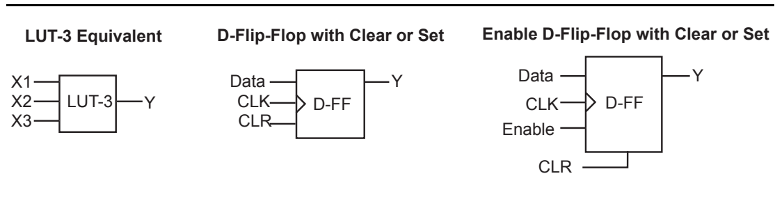
Figure 1-5 • VersaTile Configurations
