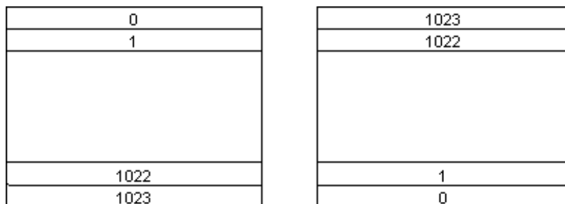
Figure 17. Normal and Reverse Scanning in Y
