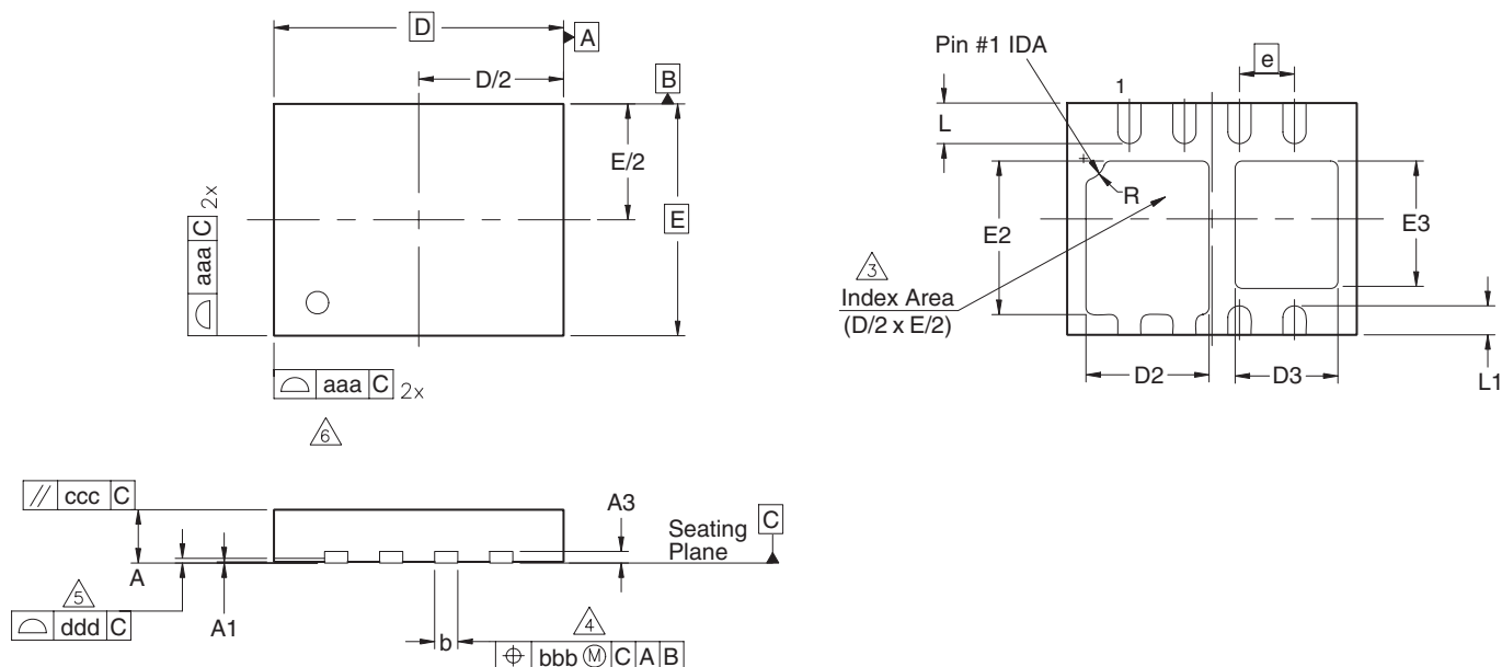
Dimensions in millimeters
