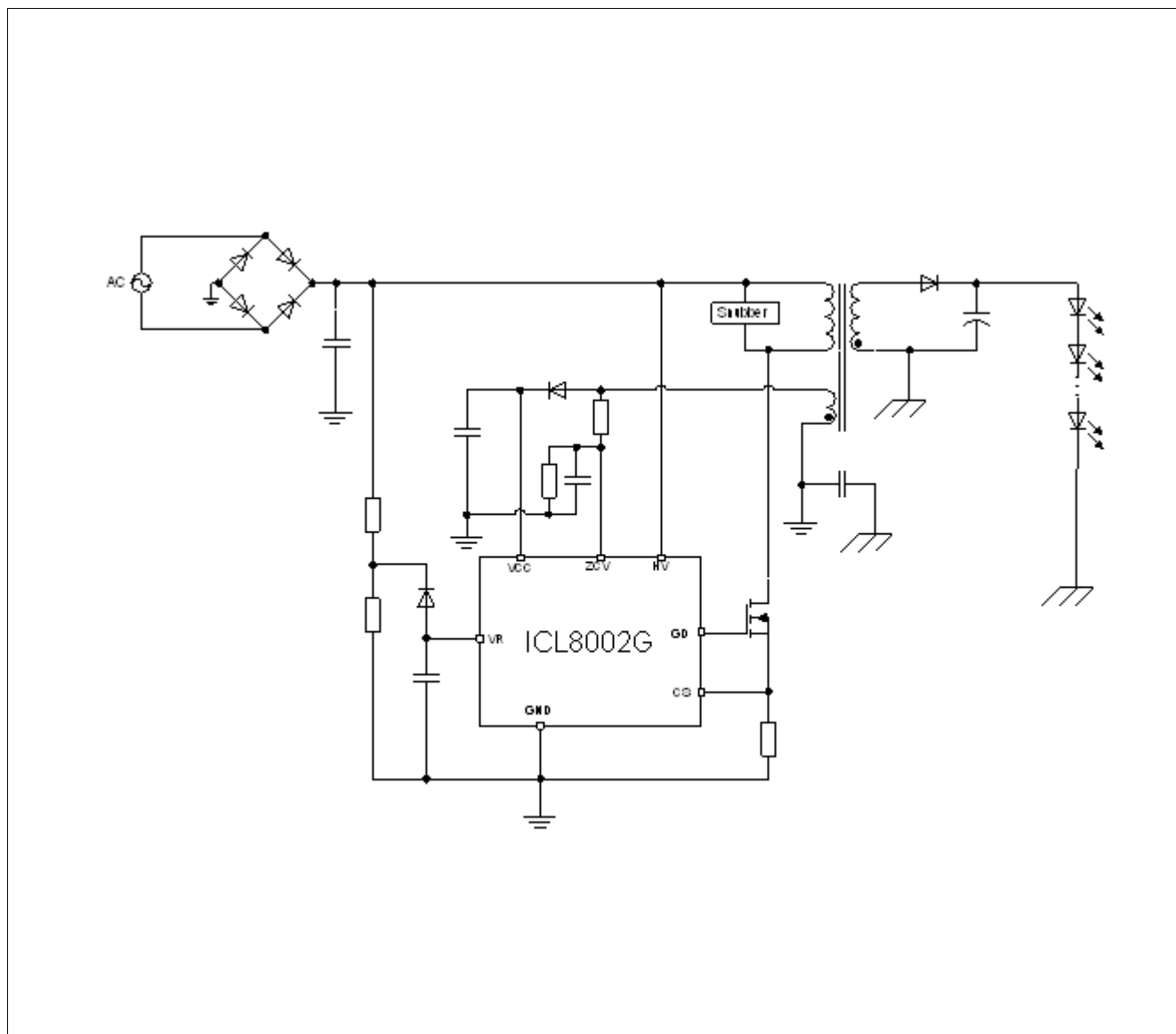
Figure 1 Application Circuit
