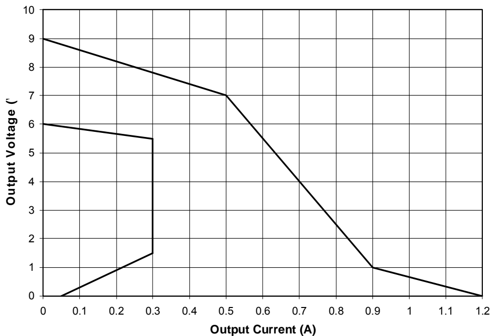
Figure 2 – Low Cost Charger Output Envelope Specification.
