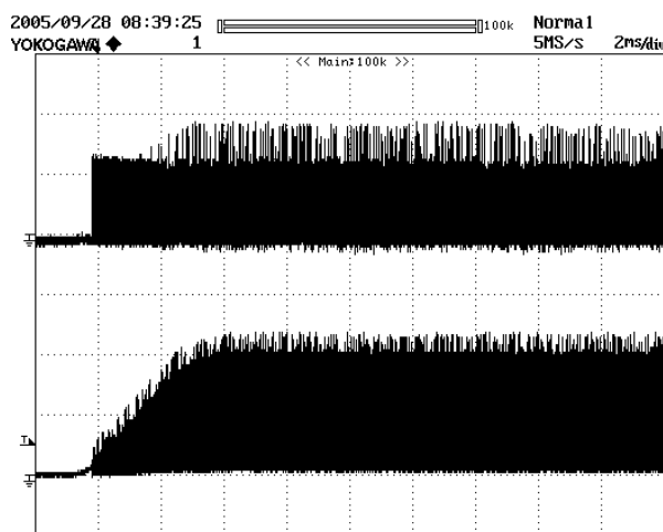
Figure 18 – 265 VAC Input and Maximum Load. Upper: I_{DRAIN} , 0.10 A / div. Lower: V_{DRAIN} , 200 V, 2 ms / div.
