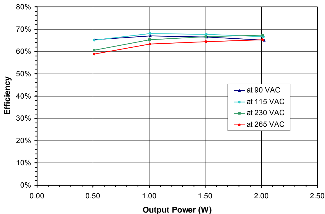
Figure 8 — Efficiency vs. Output Power.
