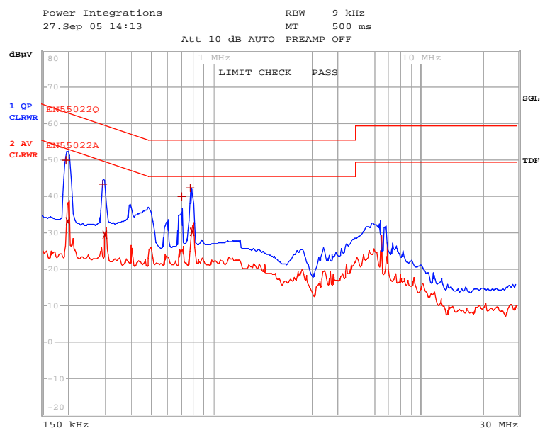
Figure 24 – Conducted Emissions, Line 115 VAC, 17 \Omega Load, with Artificial Hand at Output. QP-Dark Blue, AVG-Red.
