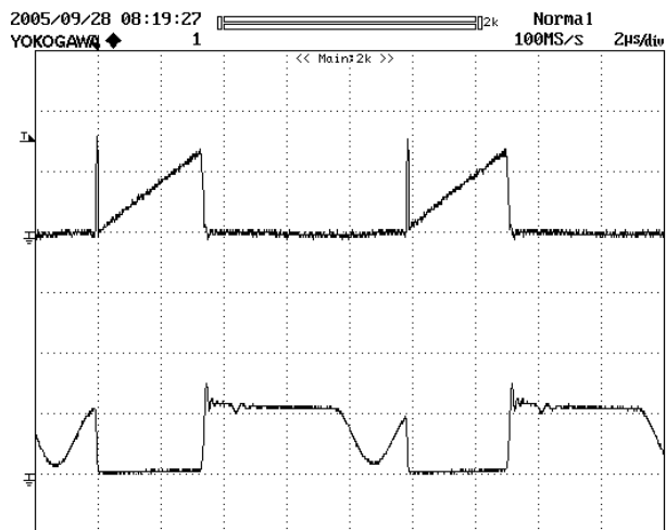
Figure 12 – 90 VAC, Full Load.
