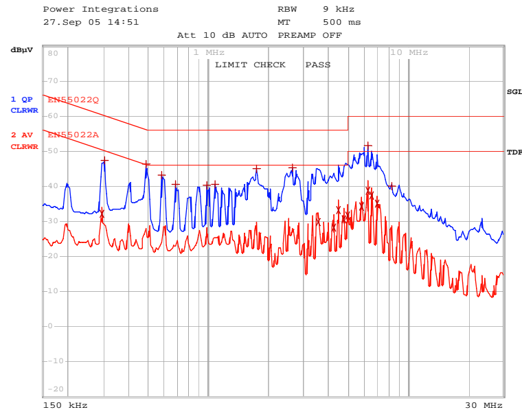
Figure 25 – Conducted Emissions, Neutral 230 VAC, 17 \Omega Load, with Artificial Hand at Output. QP-Dark Blue, AVG-Red.
