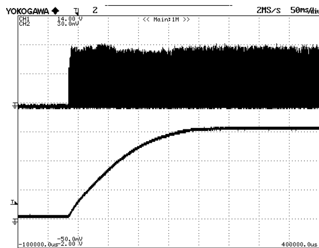
Figure 14 – Battery Output Load, R_{LOAD} = 15 \Omega .
