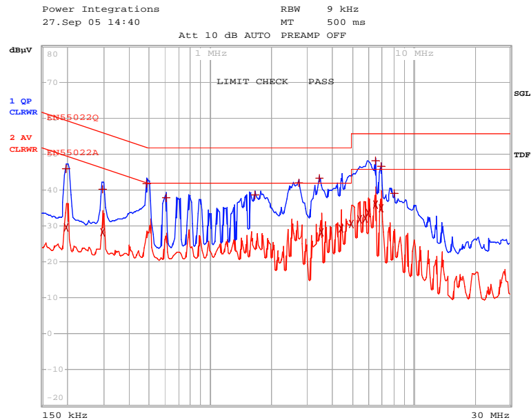
Figure 23 – Conducted Emissions, Neutral 115 VAC, 17 \Omega Load, with Artificial Hand at Output. QP-Dark Blue, AVG-Red.
