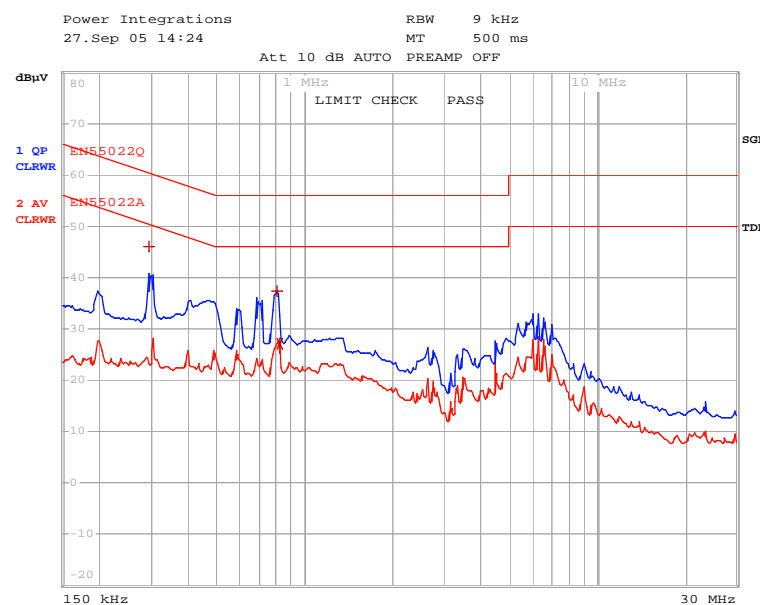
Figure 26 – Conducted Emissions, Line 230 VAC, 17 \Omega Load, with Artificial Hand at Output. QP-Dark Blue, AVG-Red
