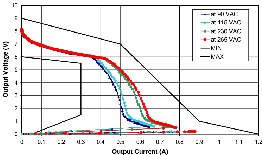
Figure 10 – Load and Line Regulation.
