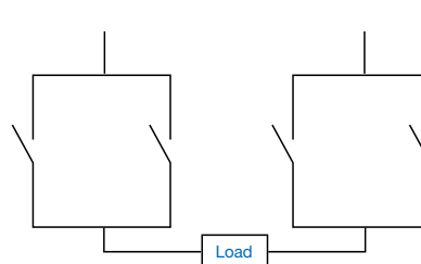
2 + 2 parallel contacts in series
