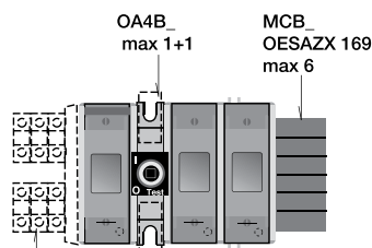
OA1G_ OA3G_ + OSZ4
