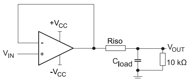
Figure 45. Test configuration for R_{ISO}
