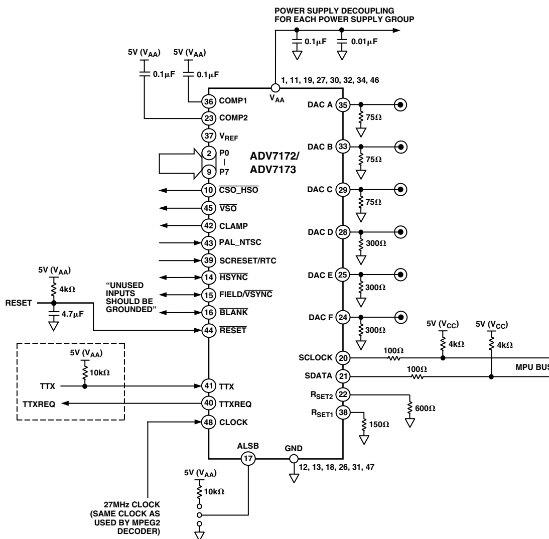
Figure 68. Recommended Analog Circuit Layout
