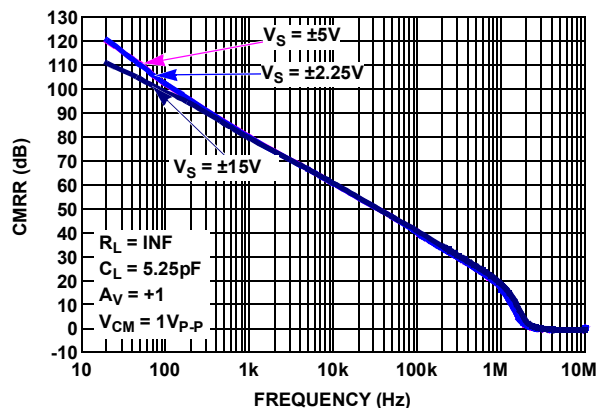
FIGURE 7. CMRR vs FREQUENCY, V_S = \pm 2.25 , \pm 5V , \pm 15V
