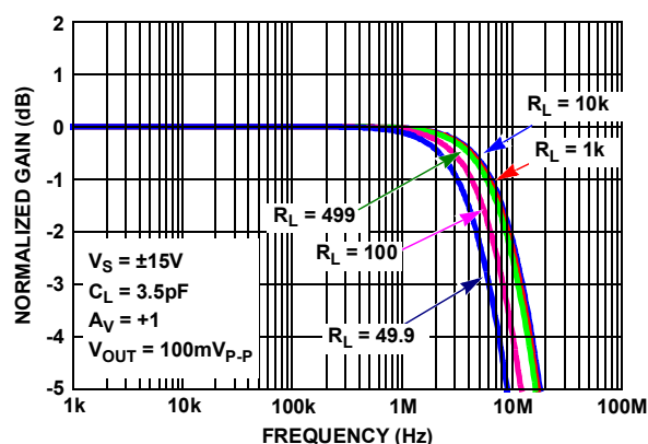
FIGURE 50. SIMULATED CLOSED LOOP GAIN vs R_L
