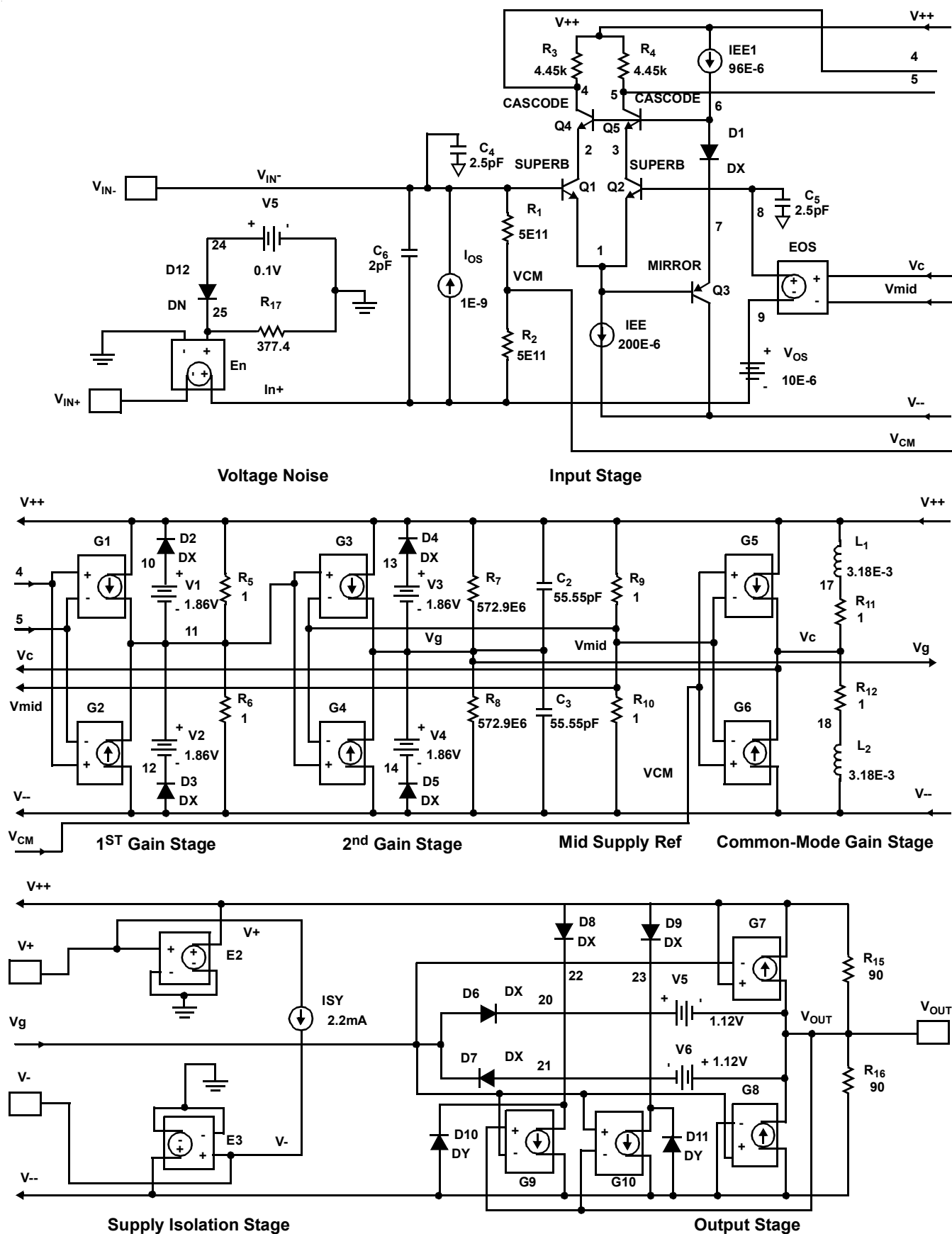
FIGURE 41. SPICE SCHEMATIC
