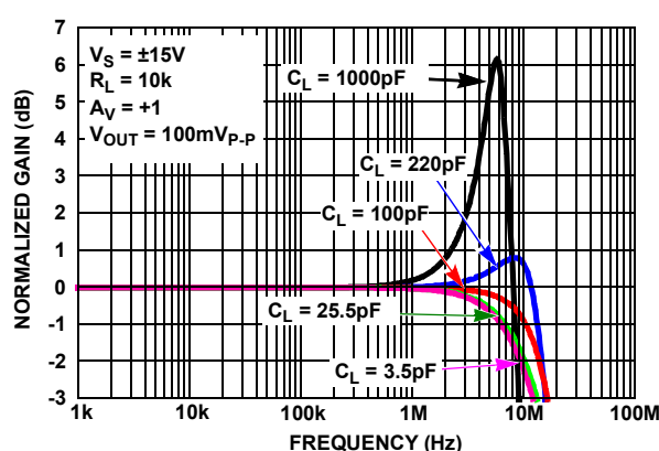
FIGURE 52. SIMULATED CLOSED LOOP GAIN vs C_L
