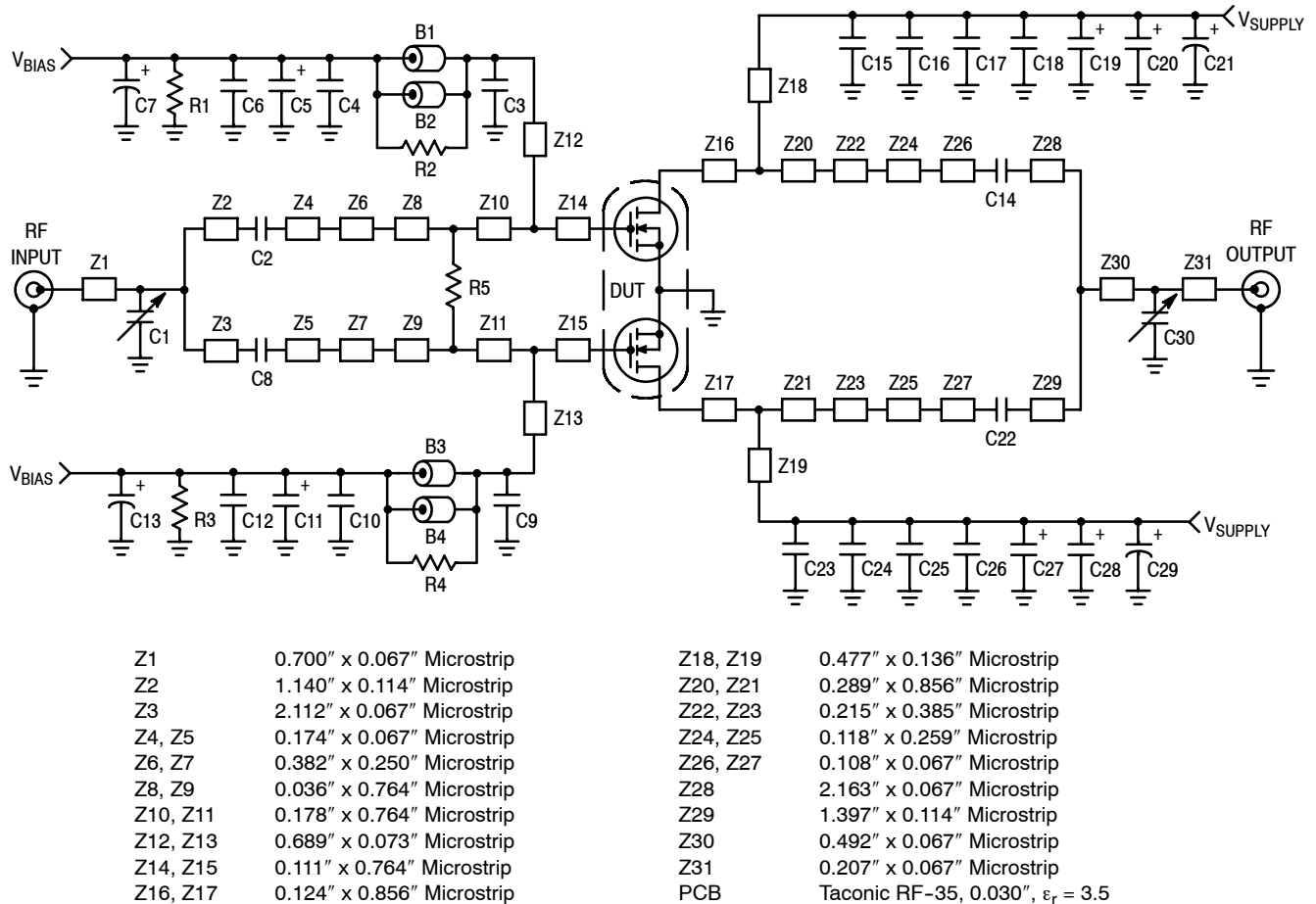
Figure 1. MRF6P18190H Test Circuit Schematic
