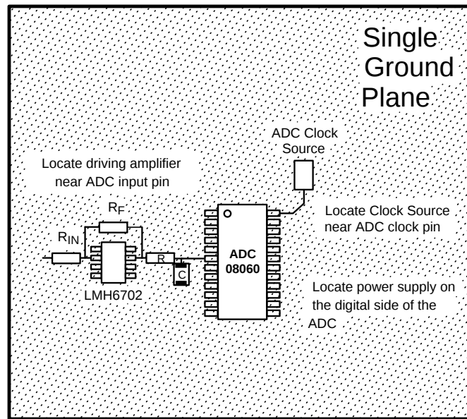
Figure 33. Layout Example
