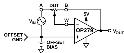
Figure 33. Test Circuit for Inverting Gain
