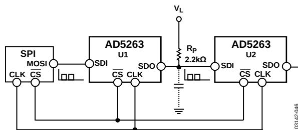
Figure 47. Daisy-Chain Configuration
