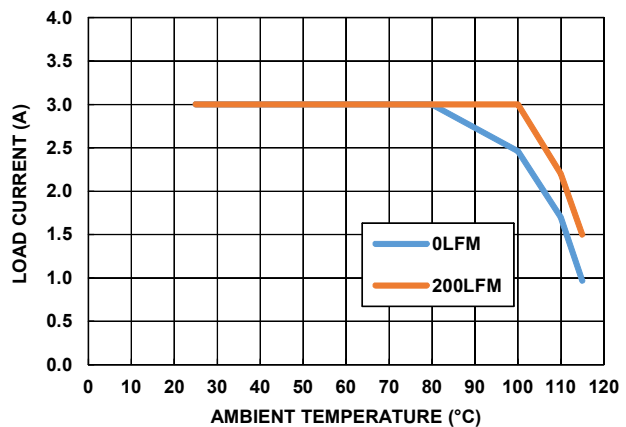
FIGURE 33. DERATING CURVES AT VIN = 3.3V, VOUT = 2.5V
