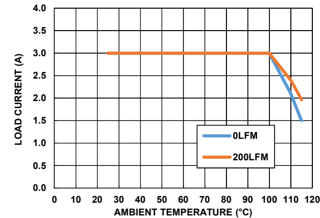
FIGURE 32. DERATING CURVES AT VIN = 3.3V, VOUT = 1.2V
