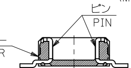
SECT.W-W(LOCK PART)
