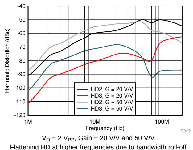
Figure 18. Harmonic Distortion vs Frequency Over Gain
