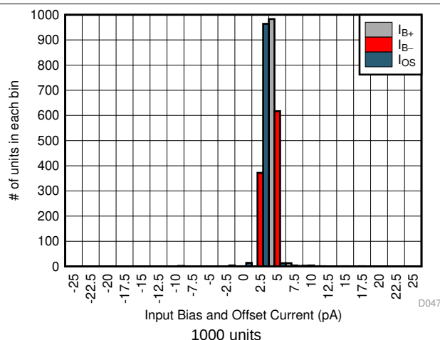
Figure 34. Input Bias and Offset Current Histogram
