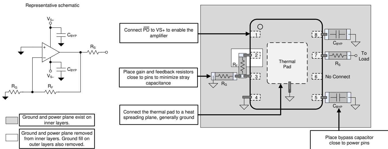
Figure 58. Layout Recommendation
