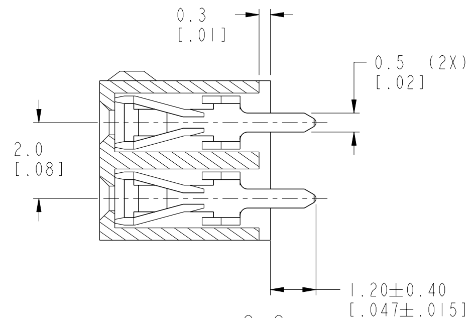
SECTION C-C
