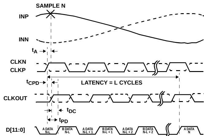
FIGURE 2. CMOS TIMING DIAGRAM—DDR (“Digital Outputs” on page 17)
