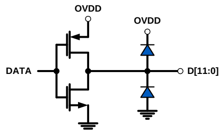
FIGURE 47. CMOS OUTPUTS
