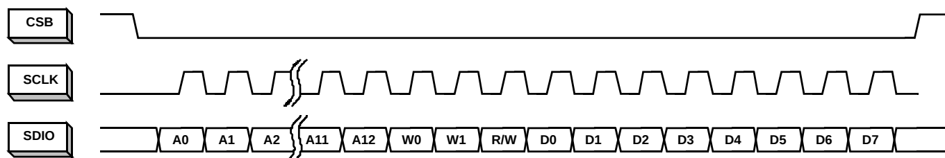
FIGURE 35. LSB-FIRST ADDRESSING
