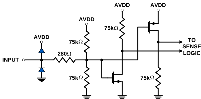
FIGURE 44. TRI-LEVEL DIGITAL INPUTS
