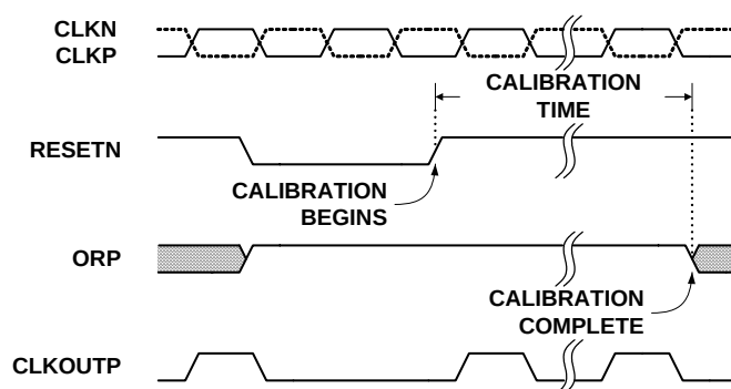
FIGURE 23. CALIBRATION TIMING
