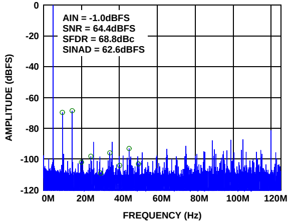
FIGURE 18. SINGLE-TONE SPECTRUM @ 495MHz
