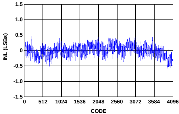
FIGURE 12. INTEGRAL NONLINEARITY
