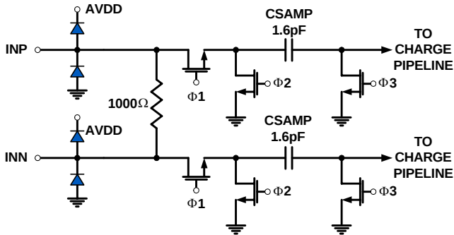
FIGURE 42. ANALOG INPUTS
