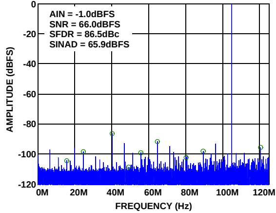
FIGURE 16. SINGLE-TONE SPECTRUM @ 105MHz
