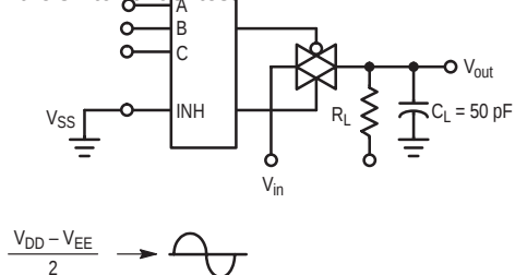
Figure 7. Bandwidth and Off-Channel Feedthrough Attenuation
