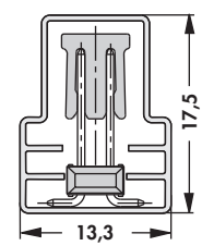
SL 11 SMD ... B SM
