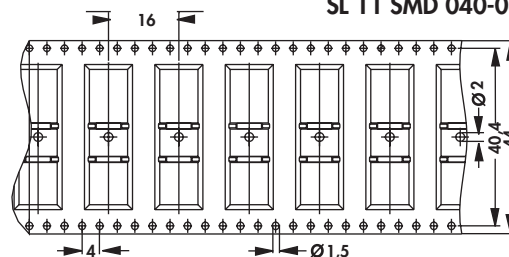
SL 11 SMD 078 ... B TR
