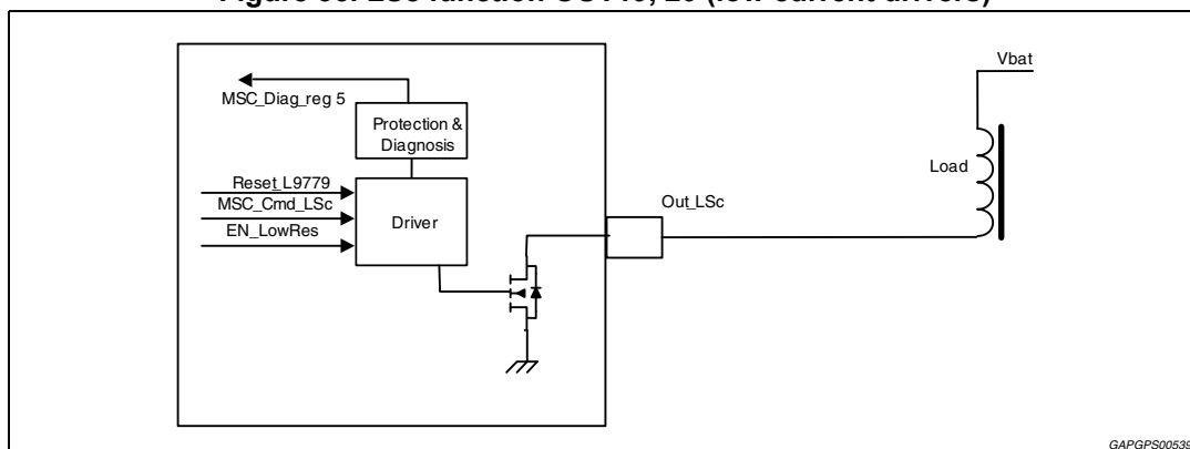
Figure 35. LSc function OUT19, 20 (low current drivers)
