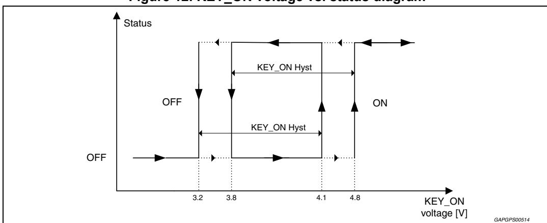
Figure 12. KEY_ON voltage vs. status diagram
