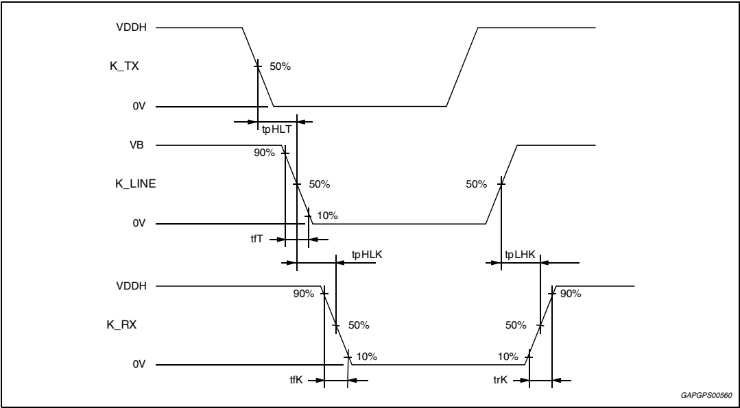
Figure 57. ISO serial line switching waveform
